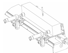
Maximum worktable profile on 3 sides tith tool (diameter 10 mm) – 60 mm height
