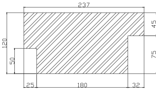
Maximum worktable profile on 2 sides tith tool (diameter 10 mm) – 60 mm height
