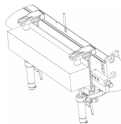
Maximum worktable profile on 1 sides tith tool (diameter 10 mm) – 60 mm height
