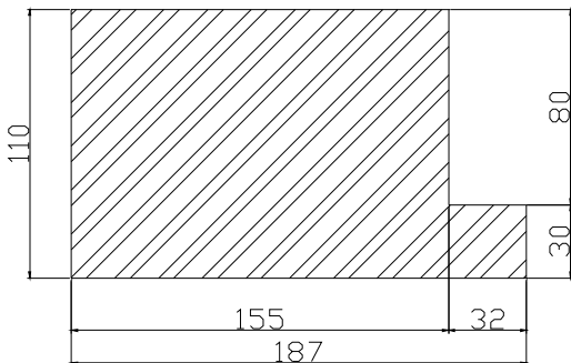
Maximum worktable profile on 2 sides tith tool (diameter 10 mm) – 60 mm height
