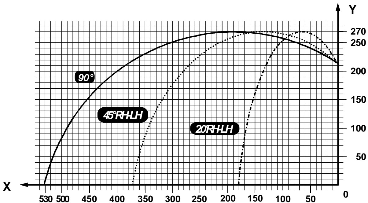
Cutting diagram
